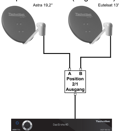
Beispiel 1: 2 Satelliten (Single-LNBs)
