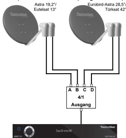
Beispiel 2: 4 Satelliten (Single-LNBs)
